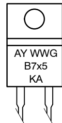
TO-220AC CASE 221B STYLE 1
