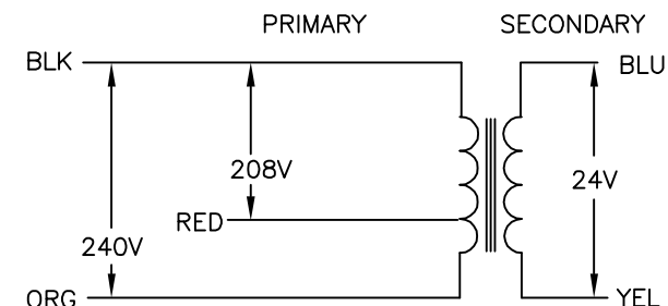
SCHEMATIC
