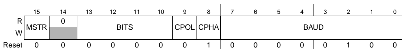
Figure 22-2. QSPI Mode Register (QMR)
