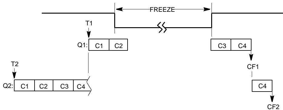
Figure 28-41. CCW Freeze Situation 19
