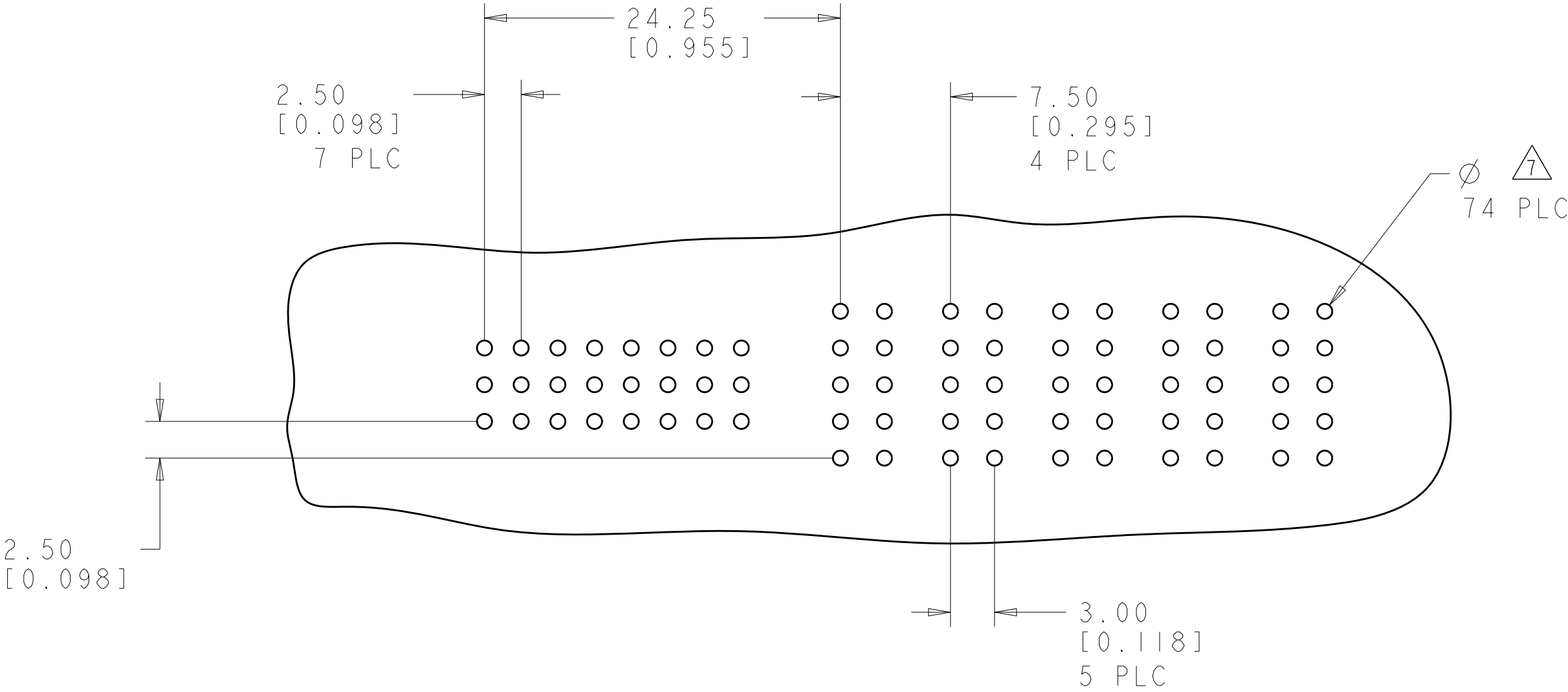
PRINTED CIRCUIT LAYOUT COMPONENT SIDE
