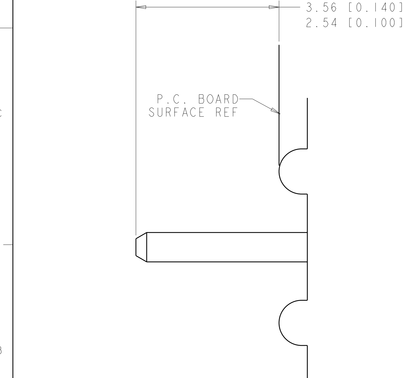
6. SOLDER TAIL DETAIL SCALE 10 : 1
