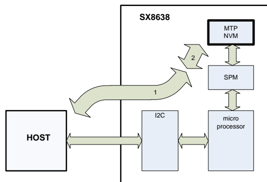
Figure 20 Host NVM mode
