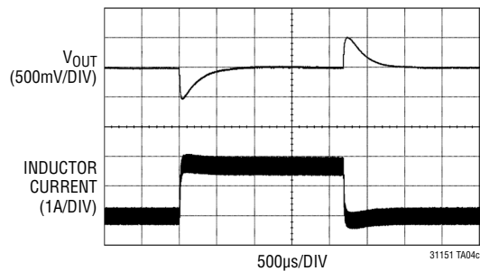
0A to 1.5A Load Step, V_{IN} = 24V
