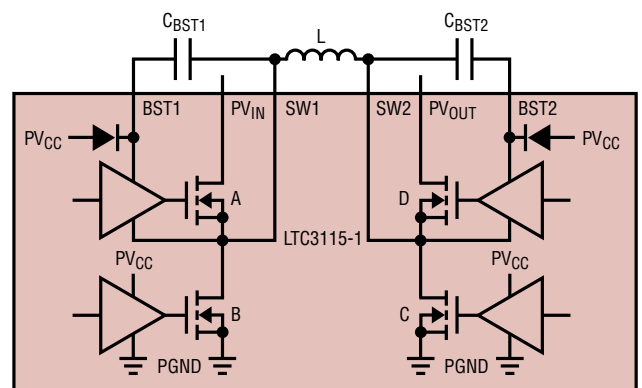
Figure 1. Power Stage Schematic
