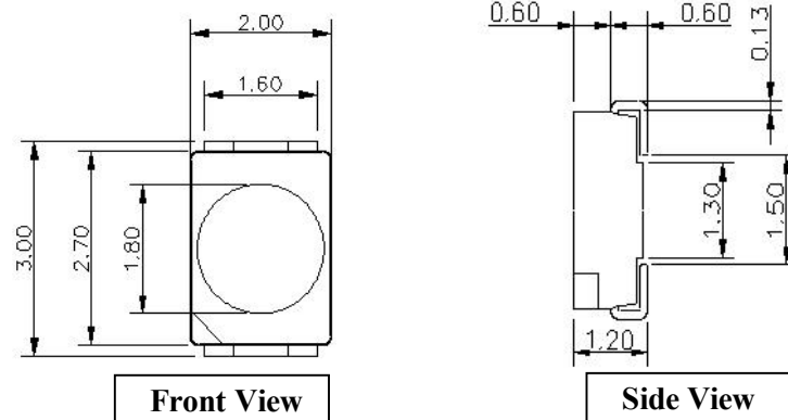
Package Outlines
