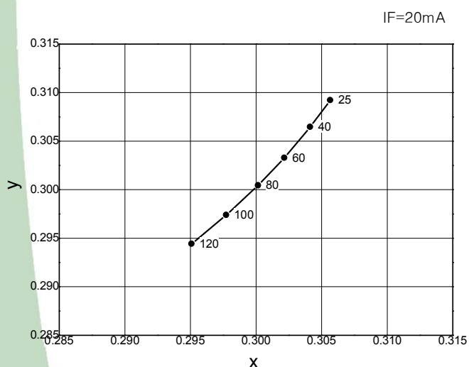
Junction Temperature ( ^{\circ}\text{C} ) vs. Chromaticity Coordinate
