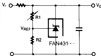
Figure 5. Shunt Regulator
