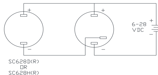
Wiring Diagram
