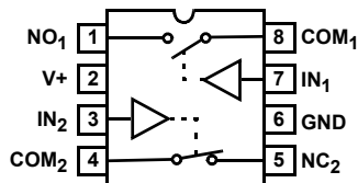
ISL84544 (SOT-23) TOP VIEW
