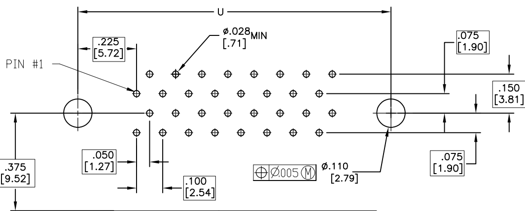
RECOMMENDED PRINTED CIRCUIT BOARD LAYOUT (CONNECTOR SIDE)
