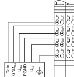
Connection diagram
