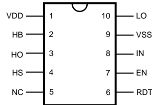
10-Pin VSSOP (DGS), WSON (DPR) Top View
