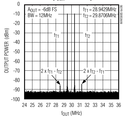
TWO-TONE INTERMODULATION DISTORTION ( f_{CLK} = 100MHz )
