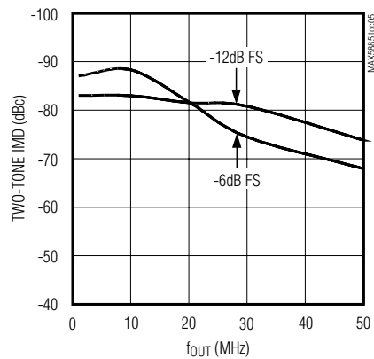
TWO-TONE IMD vs. OUTPUT FREQUENCY (1MHz CARRIER SPACING, f_{CLK} = 100MHz )
