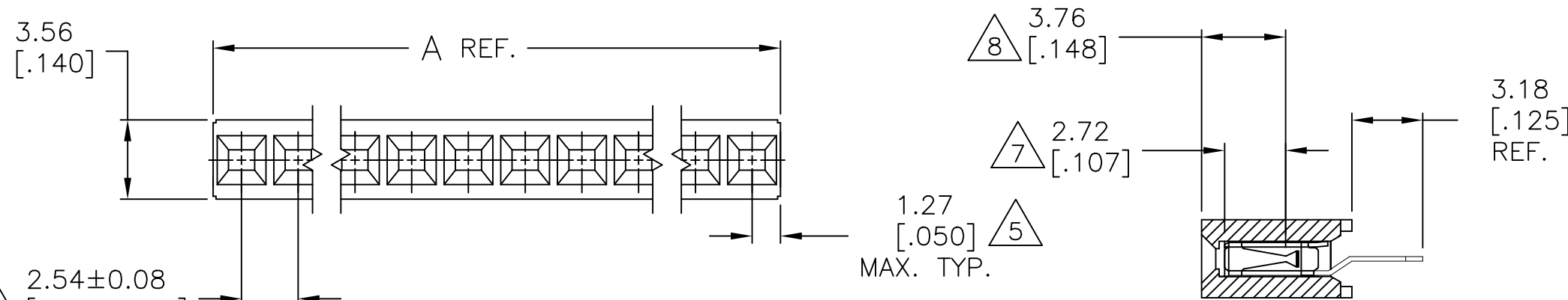
SECTION X-X
