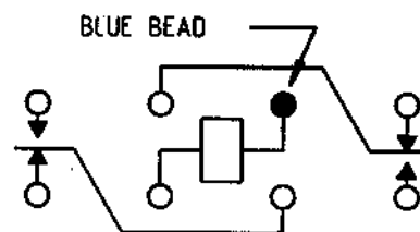
TERMINAL VIEW
