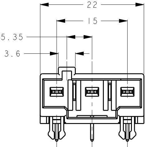
3-2229803-1 (3POSN KEYING: X)
