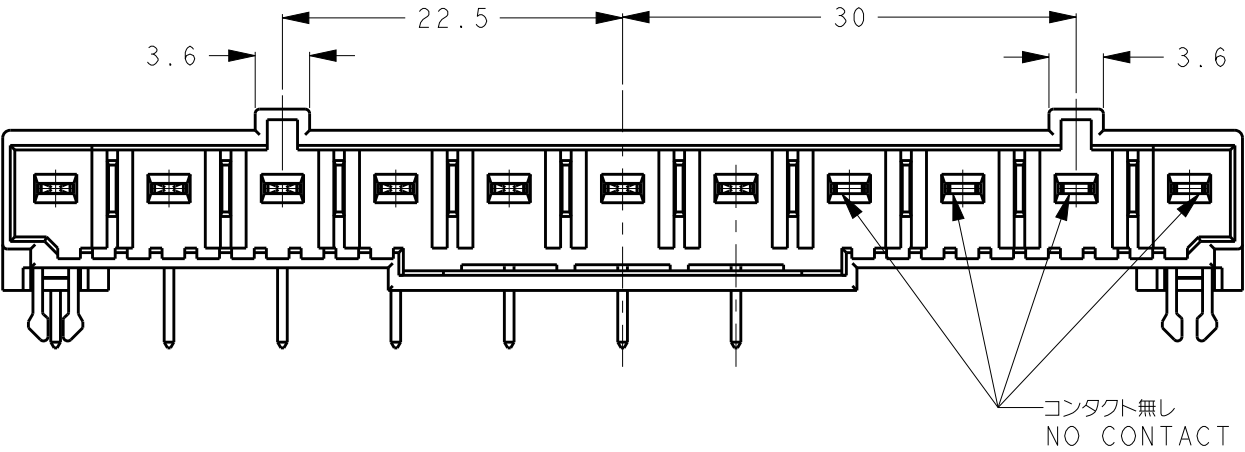
1-2229803-2 (7POSN KEYING: Y)
