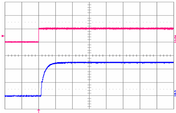
Figure 6. Turn-on transient at full rated load current (resistive) with C_o = 1\mu\text{F cer} + 10\mu\text{F tant} at V_{in} = 48\text{ V} , triggered via ON/OFF pin. Top trace: ON/OFF signal (5 V/div.). Bottom trace: Output voltage (1.0 V/div.). Time scale: 5 ms/div.
