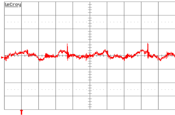
Figure 12. Input reflected-ripple current, i_S (10 mA/div.), measured through 10\ \mu\text{H} at the source at full rated load current and V_{in} = 48\ \text{V} . Refer to Error! Reference source not found. for test setup. Time scale: 1\ \mu\text{s}/\text{div} .
