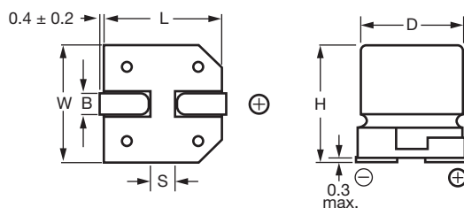
Fig. 2 - Dimensional outline
