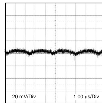
Figure 26. Output Ripple 24\text{-}V_{IN} 3.3\text{-}V_O 2A, BW = 200 MHz
