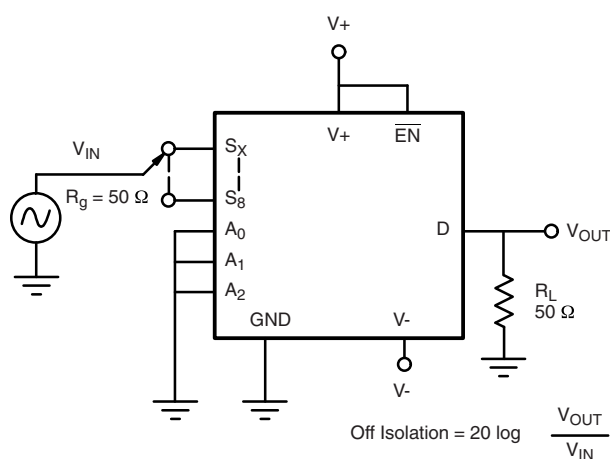
Figure 5. Off Isolation
