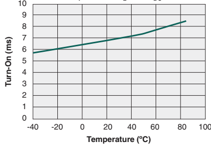
Typical Turn-On vs. Temperature ( I_F=10\text{mA} , I_L=0.4A_{DC} )
