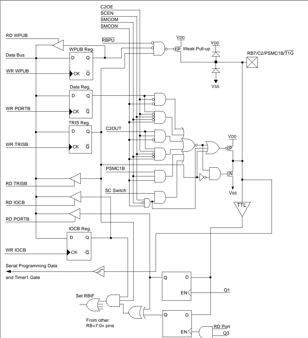
FIGURE 3-16: BLOCK DIAGRAM OF RB7/C2/PSMC1B/T1G PIN
