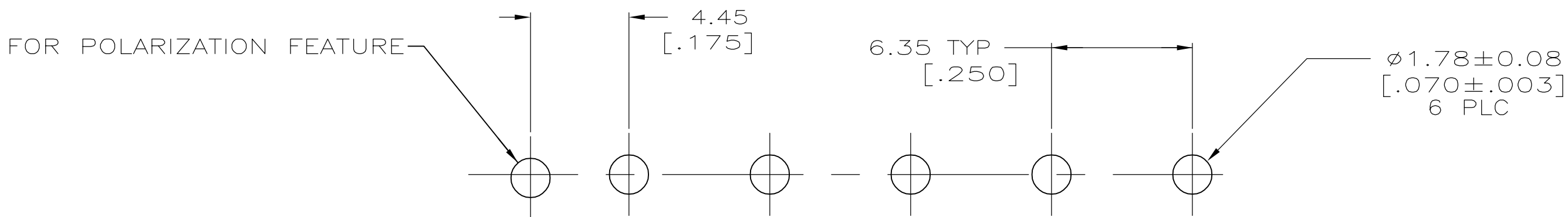
RECOMMENDED MOUNTING HOLE PATTERN FOR 1.57 [.062] THICK P.C. BOARD
