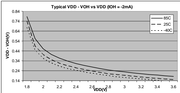
Figure 7. Typical High-Side (Source) Characteristics — Low Drive (PTxDSn = 0)
