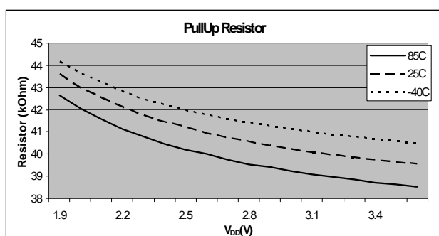
Figure 4. Pullup and Pulldown Typical Resistor Values
