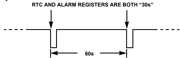
FIGURE 13. \overline{IRQ} WAVEFORM
