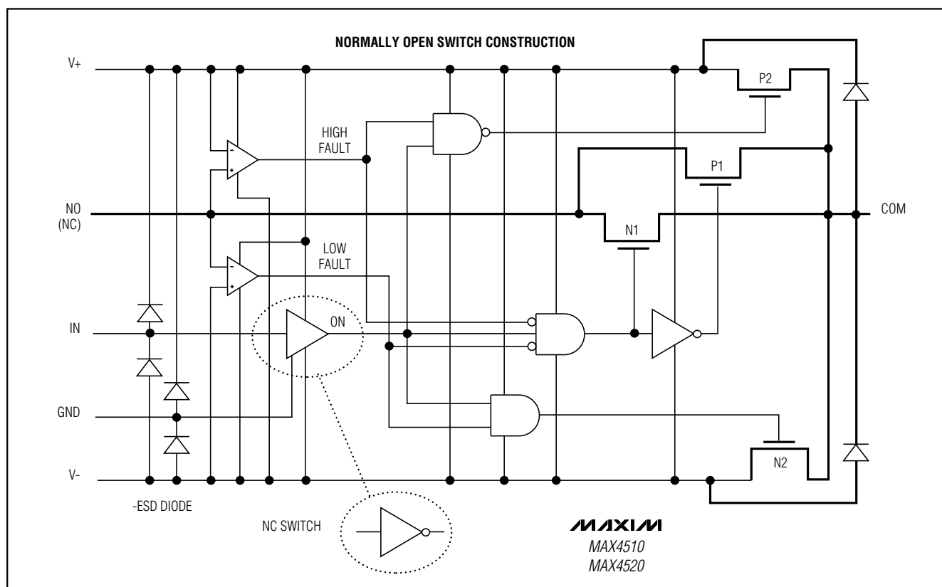
Figure 1. Functional Diagram
