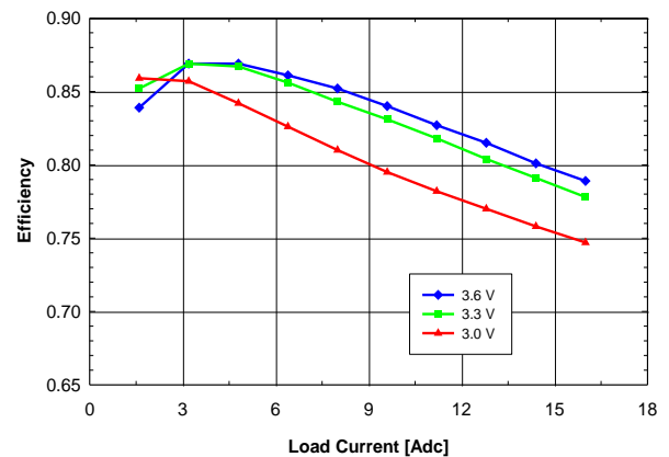
Fig. 0.7525V.3: Efficiency vs. load current and input voltage for V_{out} = 0.7525\text{ V} converter mounted vertically with air flowing from pin 10 to pin 1 at a rate of 200 LFM (1 m/s) and T_a = 25\text{ }^{\circ}\text{C} .
