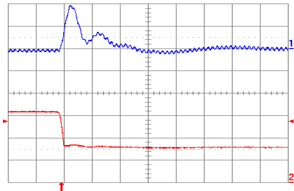
Fig. 2.5V.7: Output voltage response for V_{out} = 2.5 V to negative load current step change from 16 A to 8 A with slew rate of -5 \text{ A}/\mu\text{s} at V_{in} = 5 V. Top trace: output voltage (100 mV/div.); Bottom trace: load current (5 A/div.). C_o = 100 \mu\text{F} ceramic + 1 \mu\text{F} ceramic. Time scale: 20 \mu\text{s} /div.
