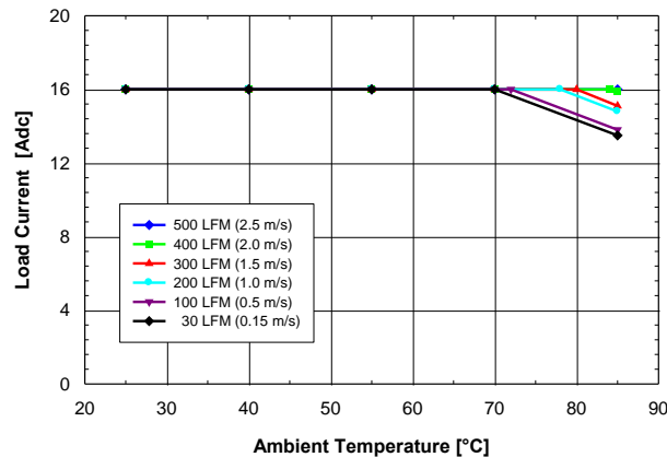
Fig. 2.5V.1: Available load current vs. ambient temperature and airflow rates for V_{out} = 2.5\text{ V} converter mounted vertically with V_{in} = 5\text{ V} , air flowing from pin 10 to pin 1, and maximum MOSFET temperature \leq 120\text{ }^{\circ}\text{C} .
