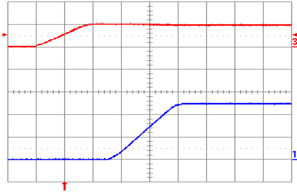
Fig. 2.5V.4: Turn-on transient for V_{out} = 2.5 V with application of V_{in} at full rated load current (resistive) and 100 \mu\text{F} external capacitance at V_{in} = 5 V. Top trace: V_{in} (5 V/div.); Bottom trace: output voltage (1 V/div.); Time scale: 2 ms/div.
