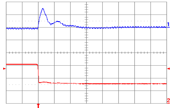
Fig. 1.5V.7: Output voltage response for V_{out} = 1.5 V to negative load current step change from 16 A to 8 A with slew rate of -5 \text{ A}/\mu\text{s} at V_{in} = 5 V. Top trace: output voltage (100 mV/div.); Bottom trace: load current (5 A/div.). C_o = 100 \mu\text{F} ceramic + 1 \mu\text{F} ceramic. Time scale: 20 \mu\text{s}/\text{div} .
