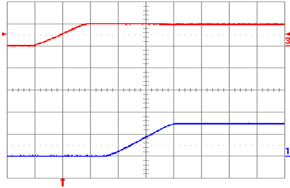
Fig. 1.5V.4: Turn-on transient for V_{out} = 1.5 V with application of V_{in} at full rated load current (resistive) and 100 \mu\text{F} external capacitance at V_{in} = 5 V. Top trace: V_{in} (5 V/div.); Bottom trace: output voltage (1 V/div.); Time scale: 2 ms/div.
