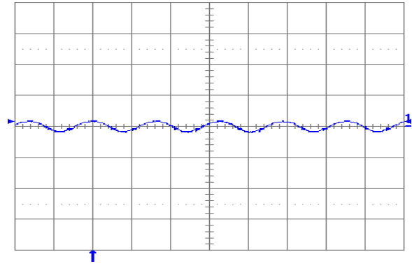
Fig. 1.5V.5: Output voltage ripple (20 mV/div.) at full rated load current into a resistive load with external capacitance 100 \mu\text{F} ceramic + 1 \mu\text{F} ceramic and V_{in} = 5 V for V_{out} = 1.5 V. Time scale: 2 \mu\text{s}/\text{div} .
