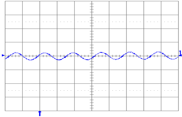
Fig. 2.5V.5: Output voltage ripple (20 mV/div.) at full rated load current into a resistive load with external capacitance 100 \mu\text{F} ceramic + 1 \mu\text{F} ceramic and V_{in} = 5 V for V_{out} = 2.5 V. Time scale: 2 \mu\text{s} /div.
