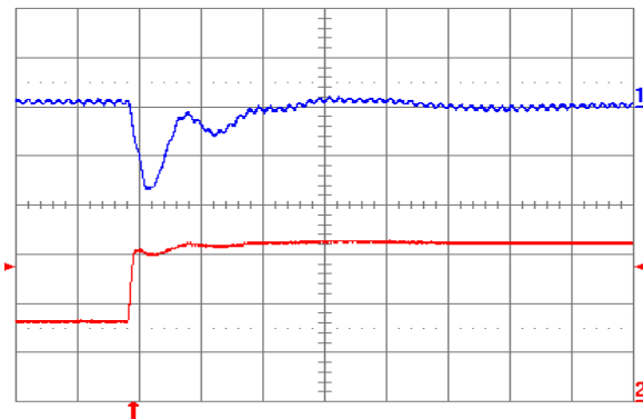
Fig. 2.0V.6: Output voltage response for V_{out} = 2.0 V to positive load current step change from 8 A to 16 A with slew rate of 5 A/ \mu s at V_{in} = 5 V. Top trace: output voltage (100 mV/div.); Bottom trace: load current (5 A/div.). C_o = 100 \mu F ceramic + 1 \mu F ceramic. Time scale: 20 \mu s/div.
