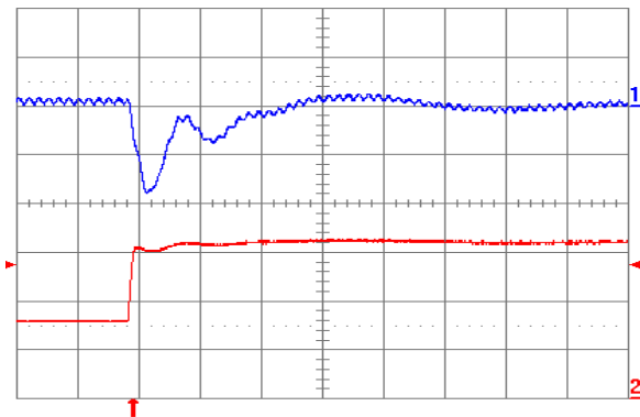
Fig. 2.5V.6: Output voltage response for V_{out} = 2.5 V to positive load current step change from 8 A to 16 A with slew rate of 5 \text{ A}/\mu\text{s} at V_{in} = 5 V. Top trace: output voltage (100 mV/div.); Bottom trace: load current (5 A/div.). C_o = 100 \mu\text{F} ceramic + 1 \mu\text{F} ceramic. Time scale: 20 \mu\text{s} /div.
