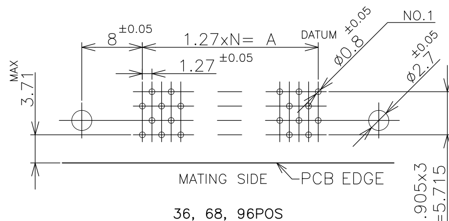
P.C. BOARD MOUNTING DIMENSIONS FIG.1
