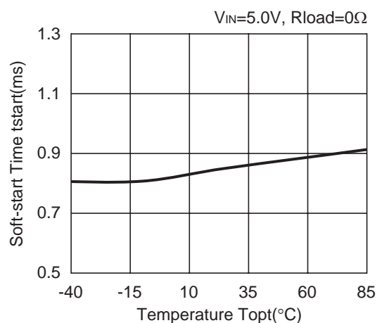
R1232D121A
