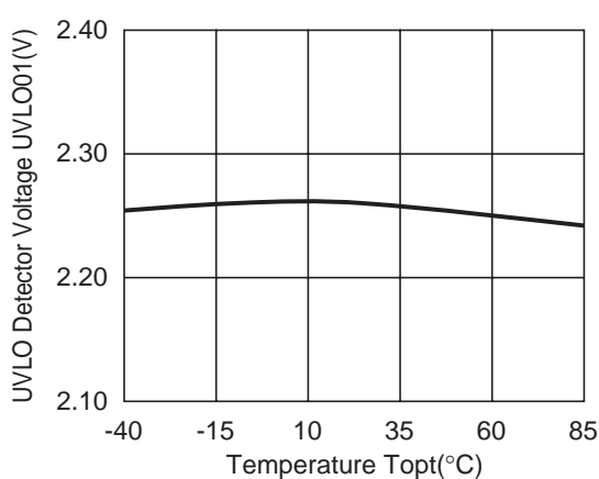
R1232D121A
