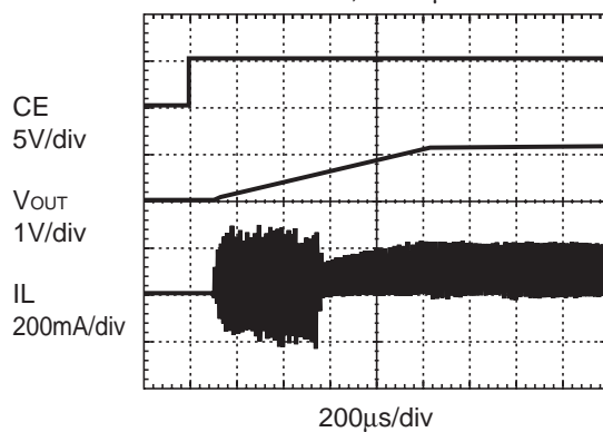
R1232D121A
