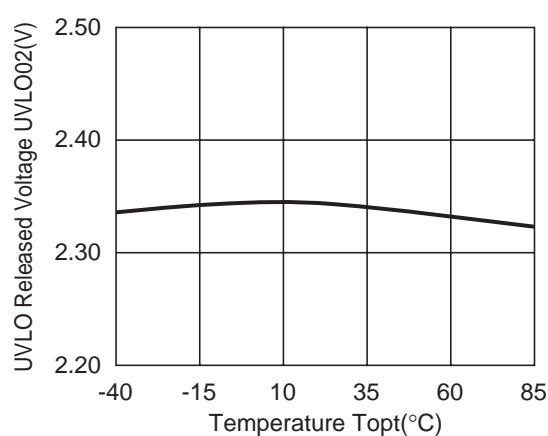
R1232D121A
