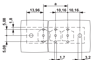
Drilling diagram
