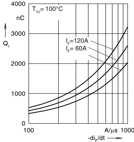
Fig. 19. Reverse recovery charge Q_r
