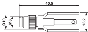
Dimensional drawing
