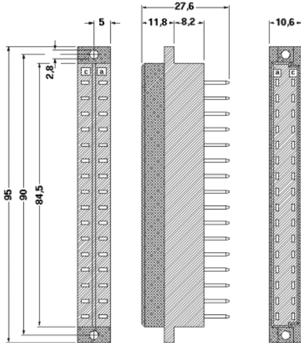
Dimensional drawing
