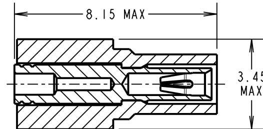
SECTION X-X
