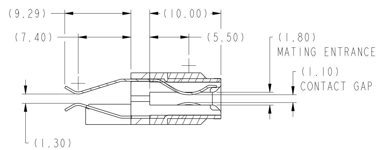
SECTION C-C
