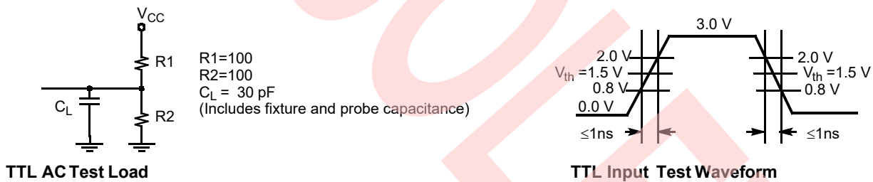
Figure 10. AC Test Loads and Waveforms
