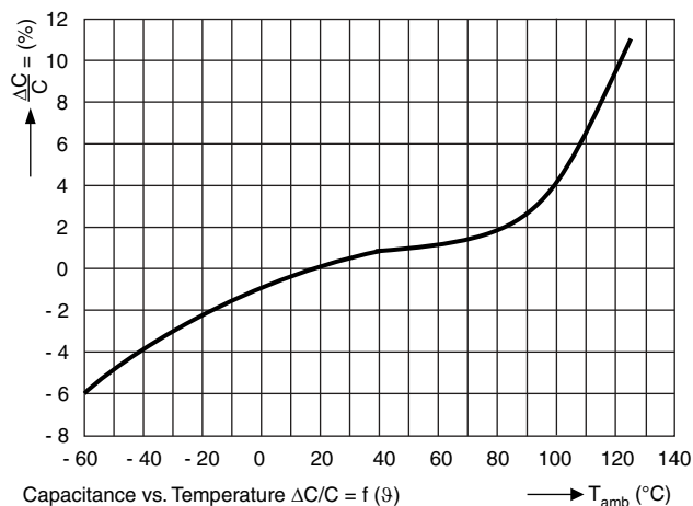
Capacitance vs. Temperature \Delta C/C = f(T_A) \Delta C/C = f(T_A), T_{LL} \leq T_A \leq T_{UL}
