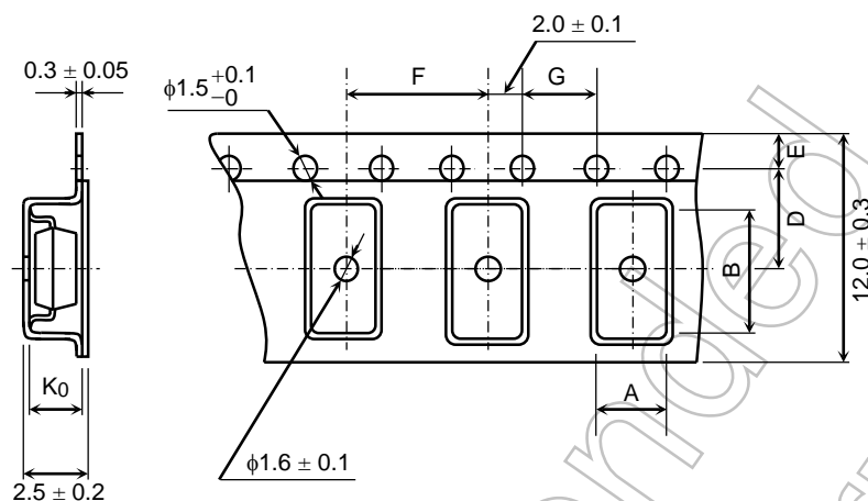
Figure 3 Tape Forms
