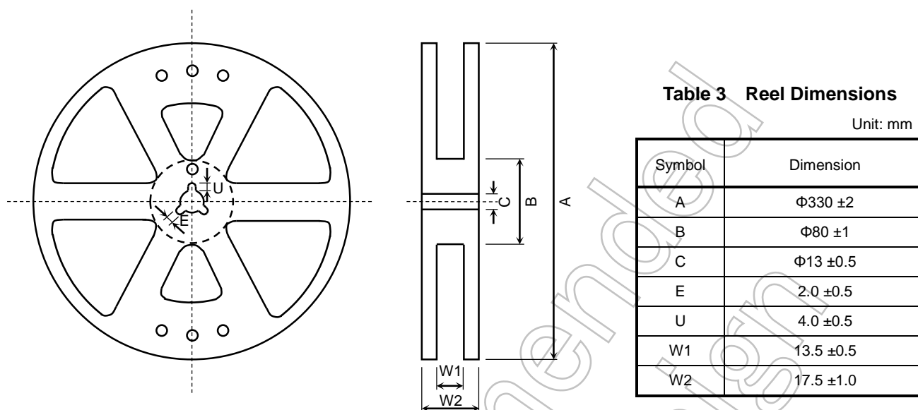
Figure 4 Reel Form
