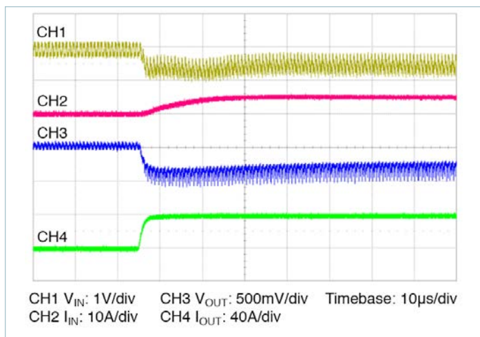
Figure 14 — 0A – 40A transient response: C_{IN} = 330\mu\text{F} , I_{IN} measured prior to C_{IN} , no external C_{OUT}
