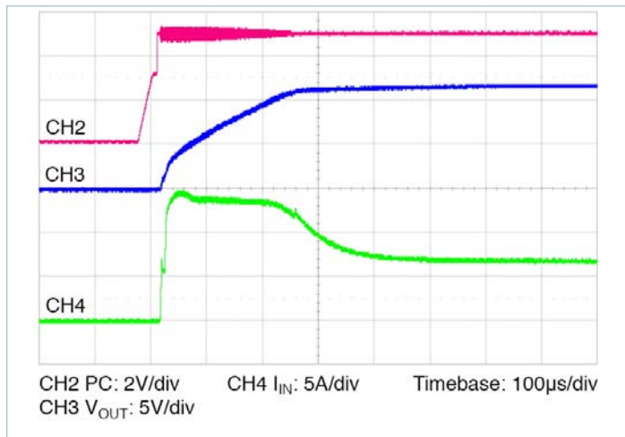
Figure 13 — Start up from application of PC; V_{IN} pre-applied C_{OUT} = 4000\mu\text{F}
