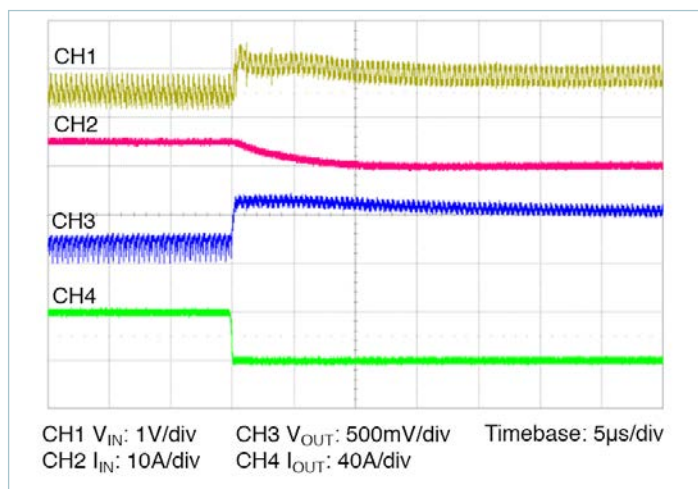
Figure 15 — 40A – 0A transient response: C_{IN} = 330\mu\text{F} , I_{IN} measured prior to C_{IN} , no external C_{OUT}
