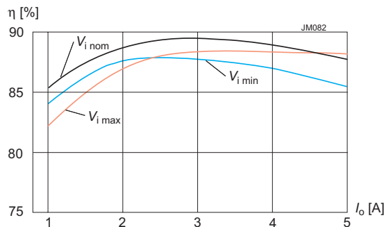
Fig. 16a Efficiency versus input voltage and current per output (BQ2320)
