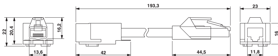
Dimensional drawing
