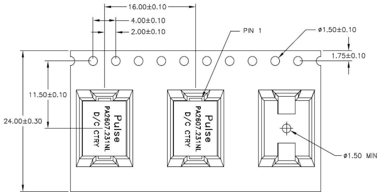
USER DIRECTION OF FEED FIGURE 1
