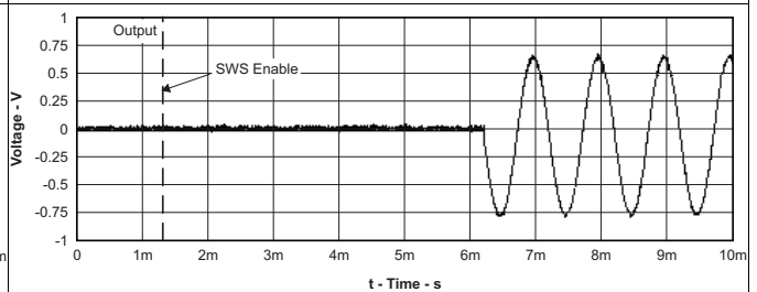
Figure 30. Start-Up Time
