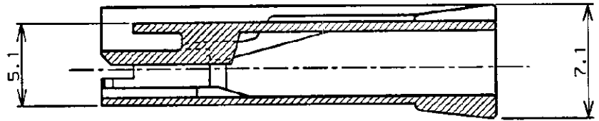
断面 "A" - "A" SECT.
