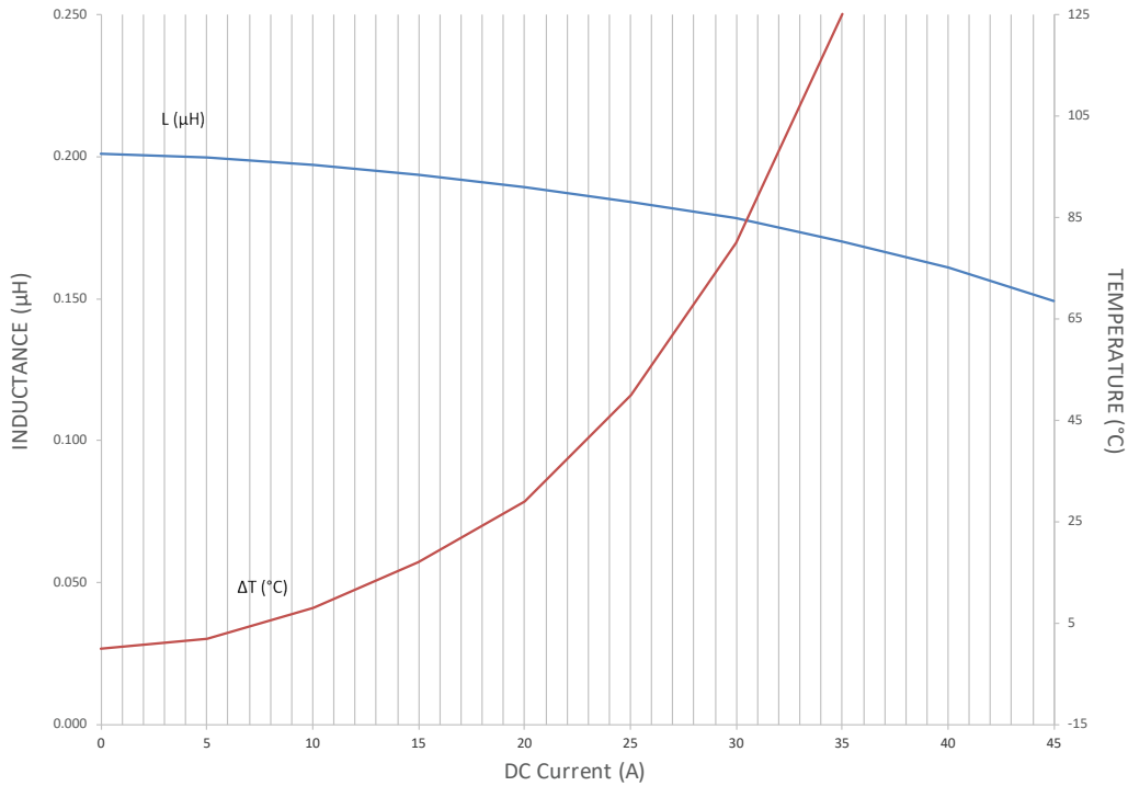
L&I Curve
