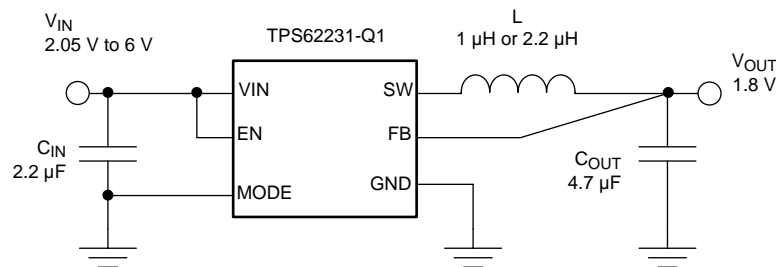
Figure 5. TPS62231-Q1 1.8-V Output
