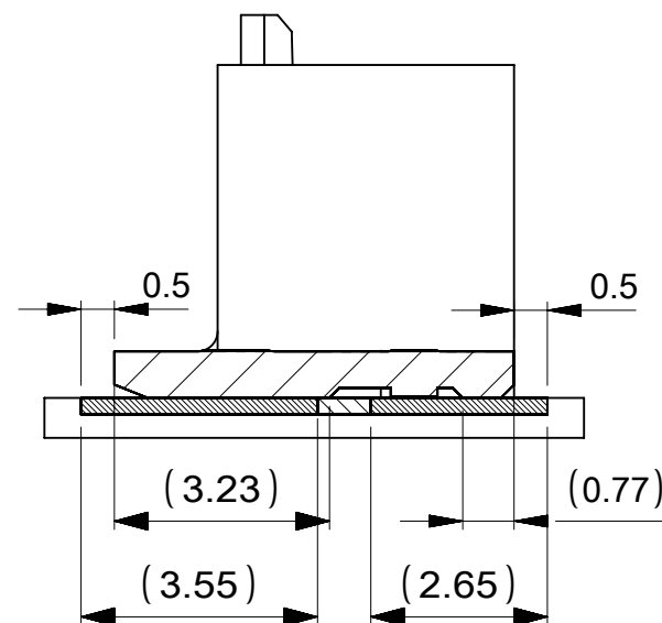
SECTION Z-Z
