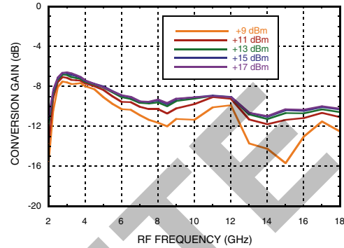
Conversion Gain vs. LO Power, IF = 100 MHz
