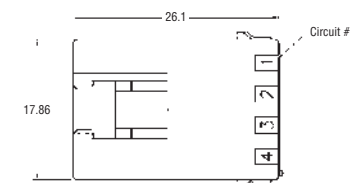
Section X-X
